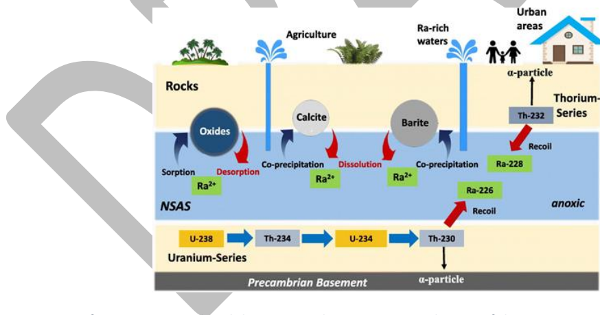
Figure 7 – Origin of Ra-isotopes and mobilization mechanism in groundwater of the Sinai peninsula (NSAS: Nubian Sandstone Aquifer; (Sherif et al. , 2018))
