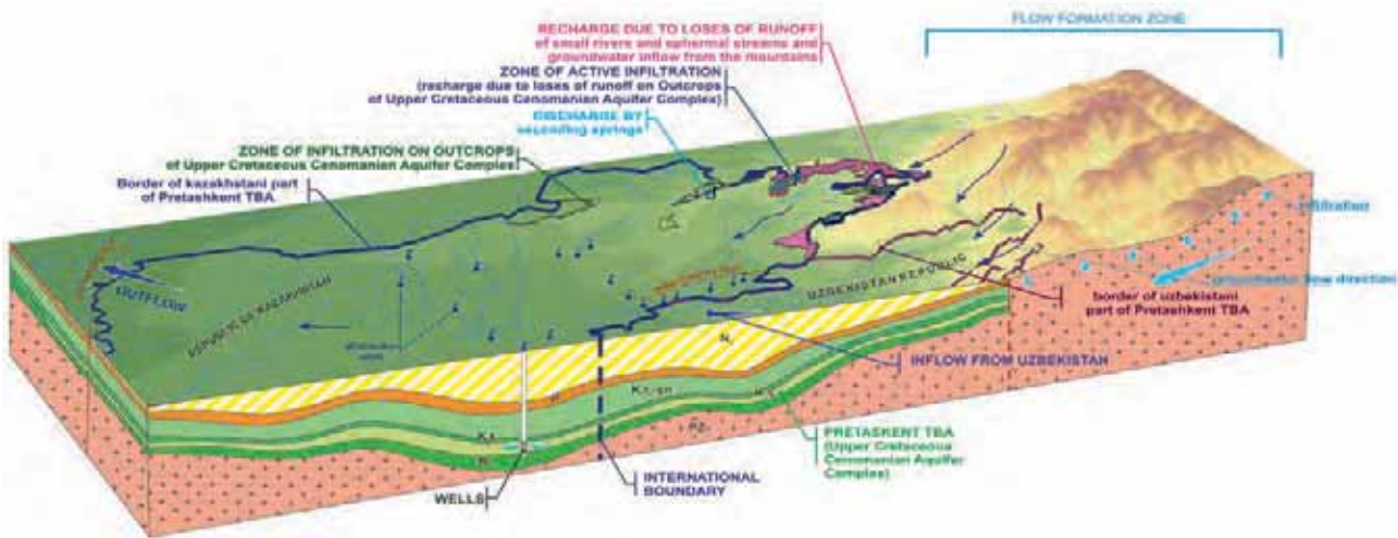
Figure 5.8 | Conceptual model of the Pretashkent Transboundary Aquifer
